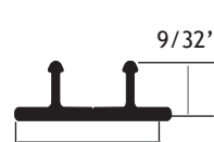
Part #110021
