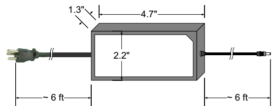
External Power Supply dimensions
