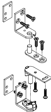
Part #570013 Brass Plated Pivot Hinge Assembly Use for light duty or covered doors, not exceeding 35 lbs.
