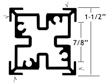
Part #170011 Corner Post Stock Length = 84"
