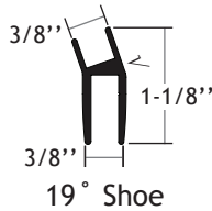
Part #110066*
