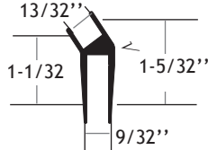
35° Deep Shoe
