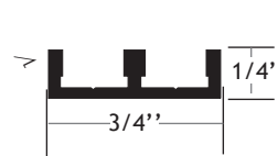
Part #110035
