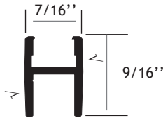
Glide Shoe
