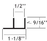
Single Channel with Extended Leg
