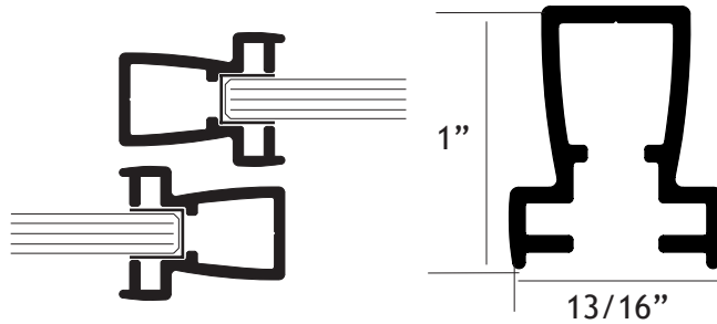
Part #130022 Wardrobe Door Header
