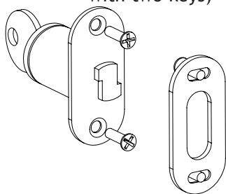
Part #530024* T-Bolt Plunger Lock (Kenstan PLD40T1 Polished Nickel with two keys)
