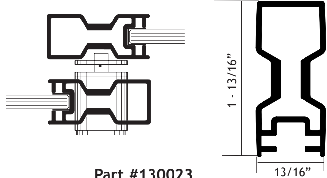
Part #130023 Wardrobe Door Track
