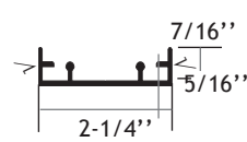
Security Track
