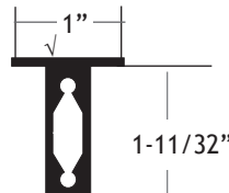
Part #110106
