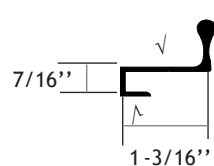
Part #110029
