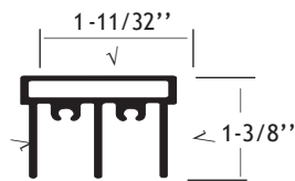
Part #110523 Backframe Header without Top Glass
