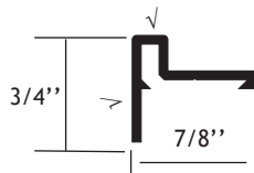
Part #110137 Cover Tee with .25 Return
