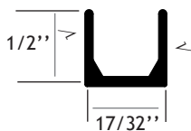
Part #110650 Front Frame for 3/8" Security Glass
