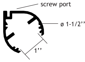
683900 series (screw port assembly)
