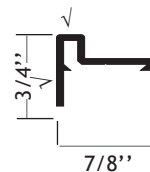
Part #110577 Showcase Molding without holes (with holes #410099)
