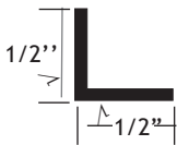
Part #110030 1/2" Angle
