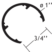
Extrusion #180133
