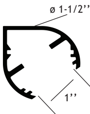
Extrusion #180147
