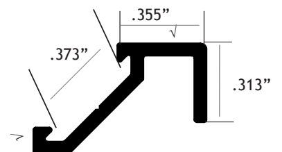
Part #110224 Glazing, Jamb w/o Leg
