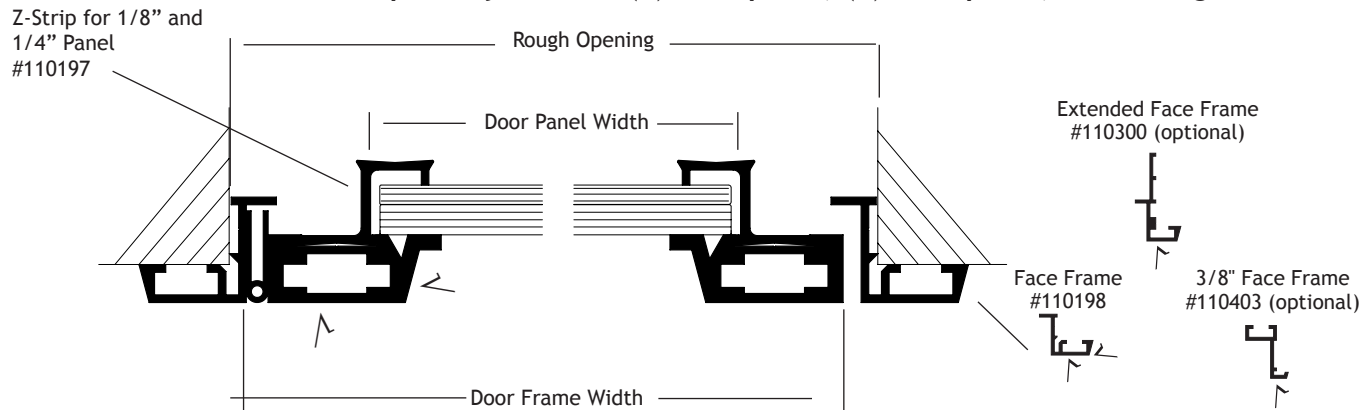
Aluminum Transparency Frame: (1) 1/8" panel, (1) 1/4" panel, Piano Hinge
