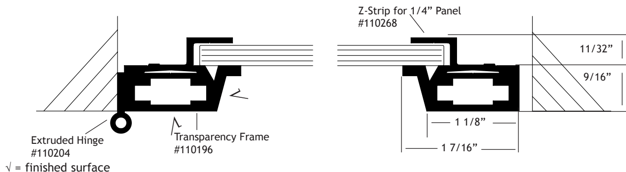
Aluminum Shadow Box Frame: (1) 1/4" panel, Extruded Hinge
