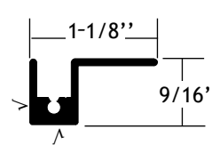
Part #110341 Edge Molding w/Leg
