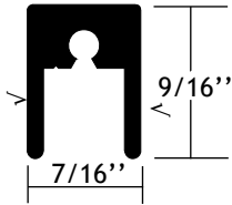
Part #110198 Z-Strip 1/2 inch Panel
