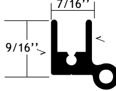
Part #110204 Heavy Duty Hinge Strip
