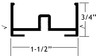
Part #170012 Jamb and Header Stock Length = 144"
