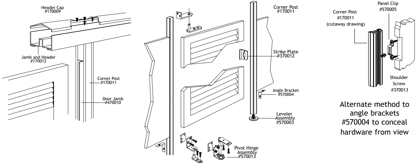
Part #170012 Jamb and Header Stock Length = 144"
