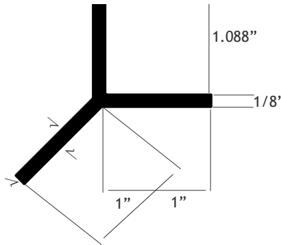
Part #111068 Y Molding
